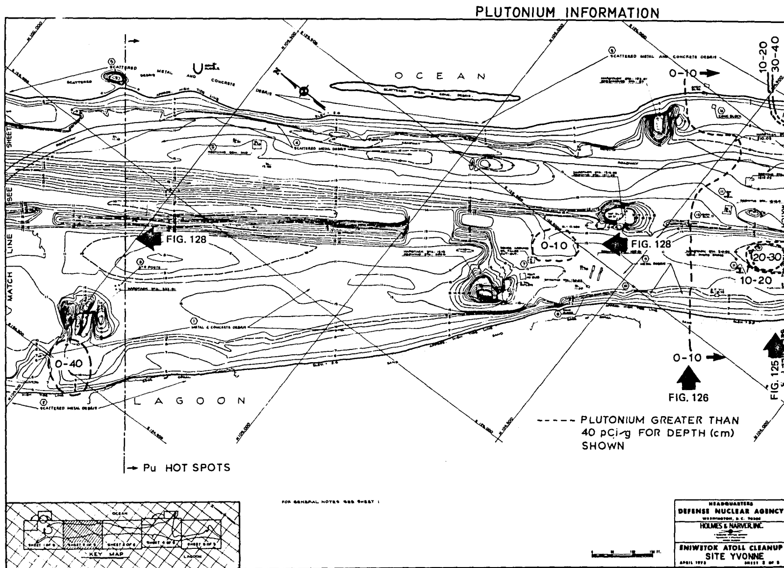
FIGURE 119. SITE YVONNE, PLUTONIUM DATA, SHEET 2 OF 5
