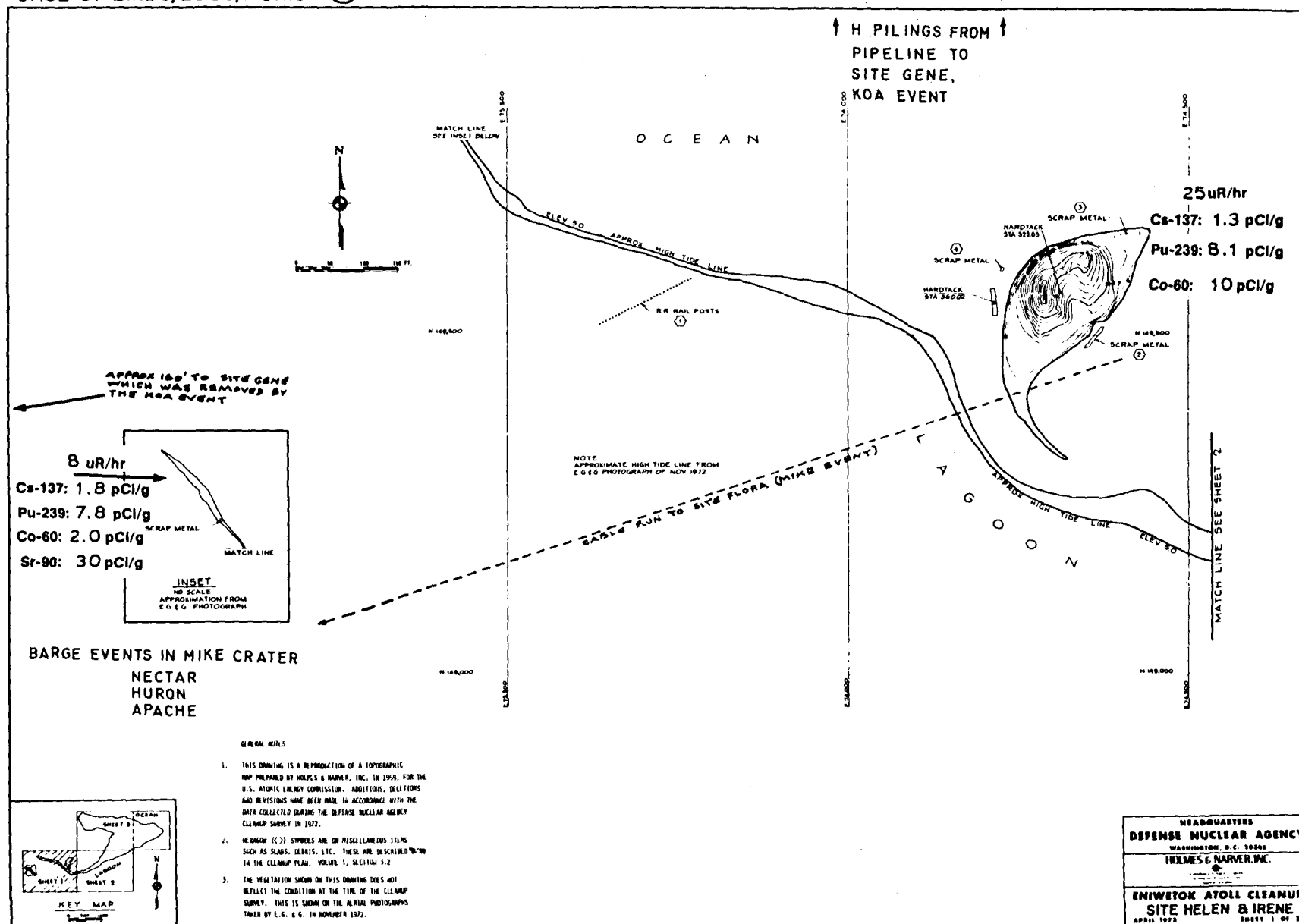
FIGURE 8. SITES HELEN AND IRENE, SHEET 1 OF 3
