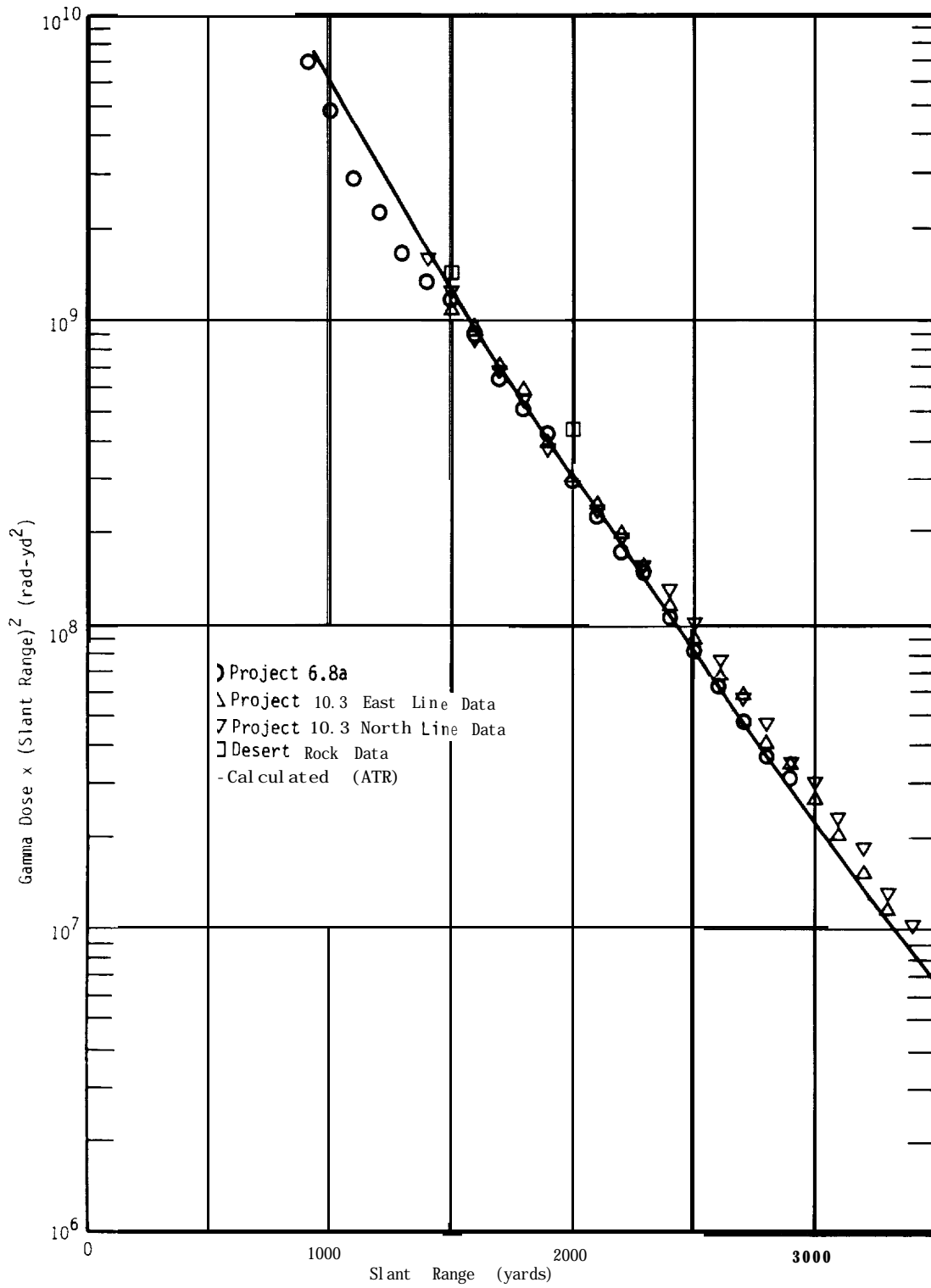
Figure 3-1 Shot Badger Initial Gamma Dose
