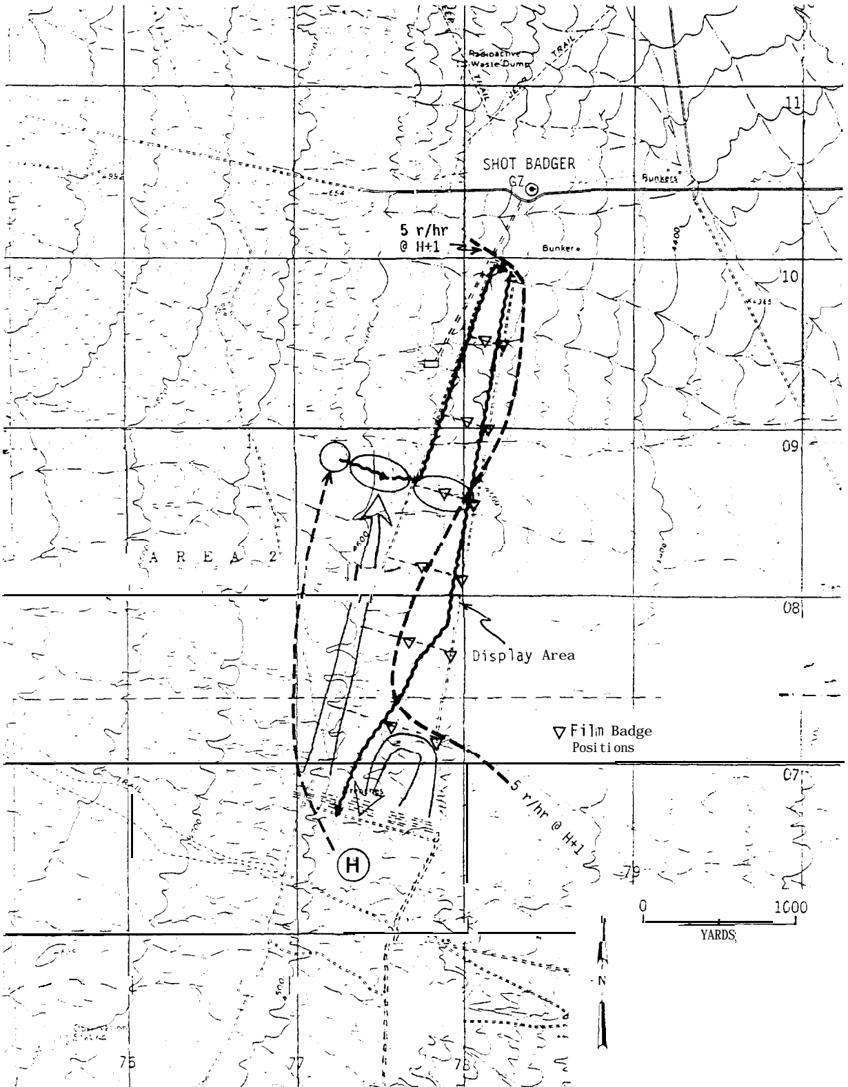
figure 4-1. Shot Badger, Residual Radiation and Troop Movements
