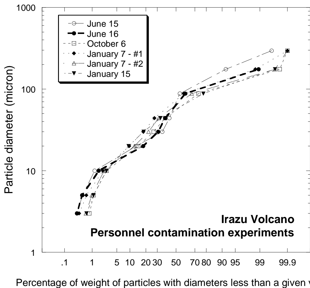
Figure 4-1. Cumulative weight distributions of volcanic ash particles in personnel contamination studies during eruption of Irazu Volcano in Costa Rica (Miller 1966b).
