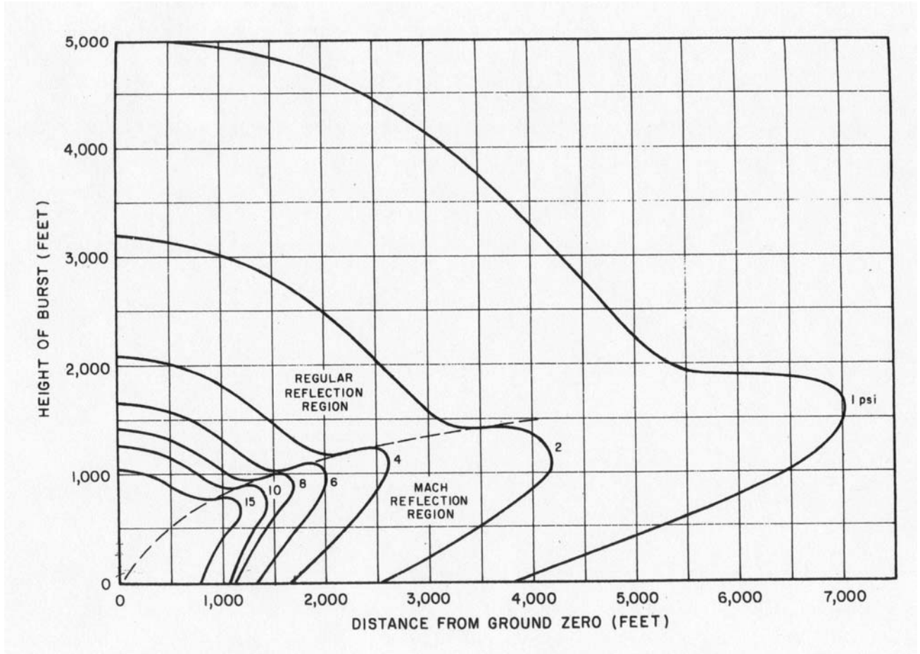
Figure 2-2. Dependence of peak overpressure at ground level in pounds per square inch (psi) on height of burst and distance from ground zero for 1-kiloton (kt) detonation (Glasstone and Dolan, 1977; Figure 3.73c). Burst height and distance of a given peak overpressure from ground zero both scale as the cube root of the yield in kt.
