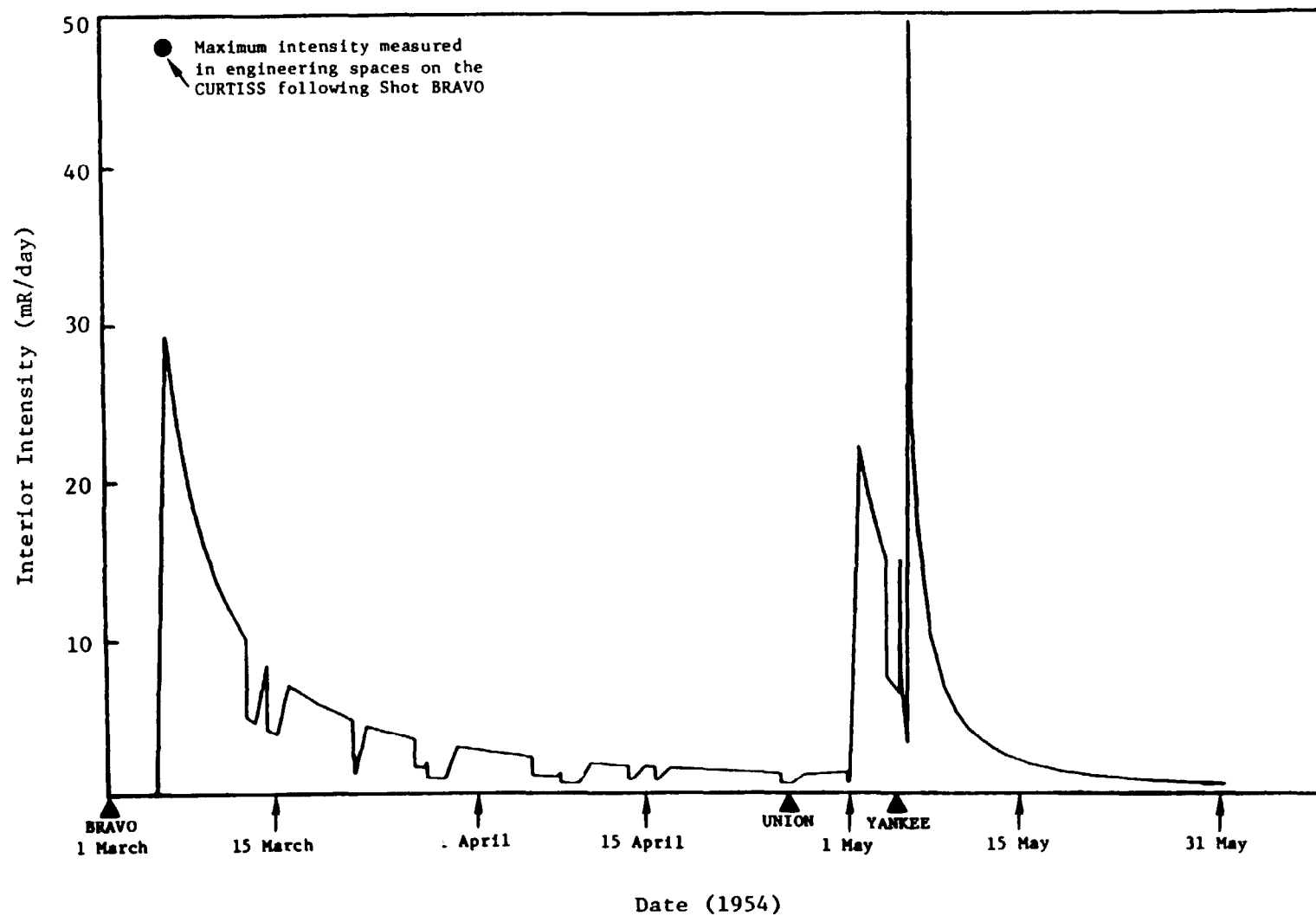
Figure 2-2. Average intensity below deck on the USS CURTISS due to ship contamination.
