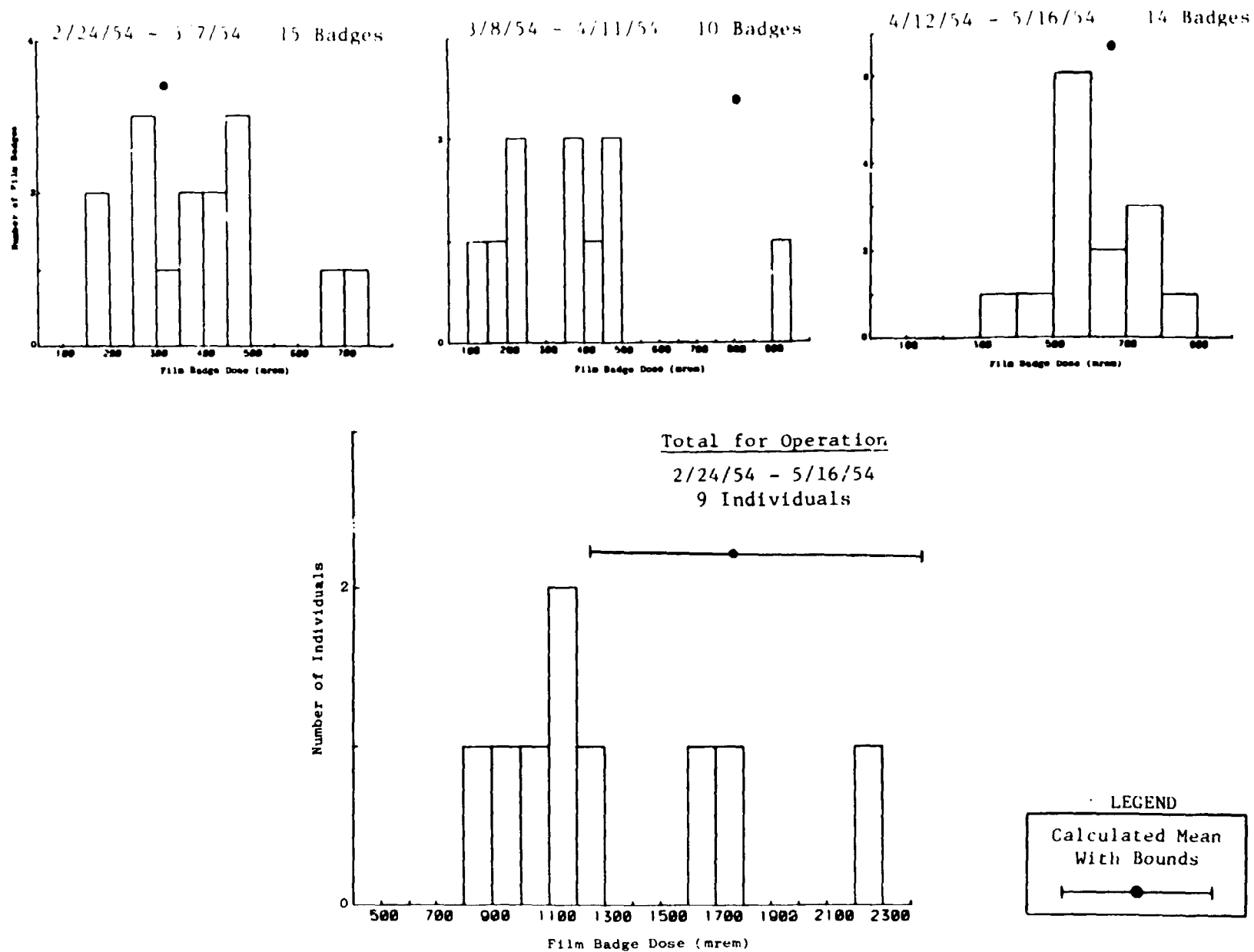
Figure 5-3. USS SIOUX - Comparison of dosimetry data with calculated doses.
