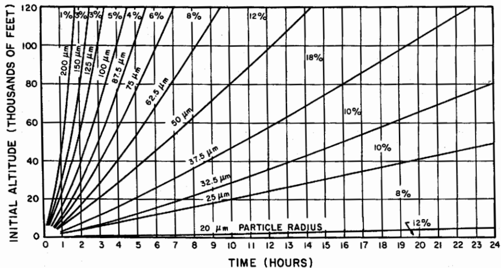
Figure 1. Fall Times of Particles of Different Sizes from Various Altitudes
